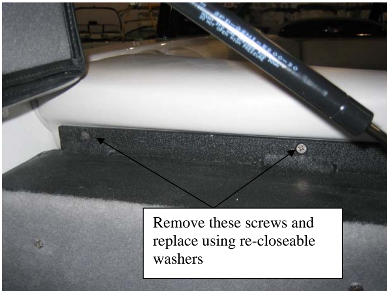
Figure 1. Location of back seat screws (10 each)
